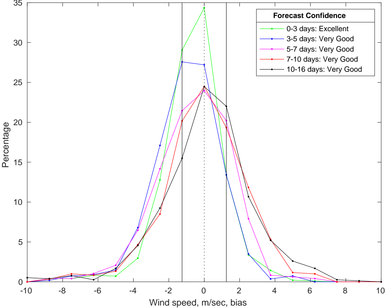
NDBC 42035 vs GFS Winds Bias Histogram: 12-Jul-2025
