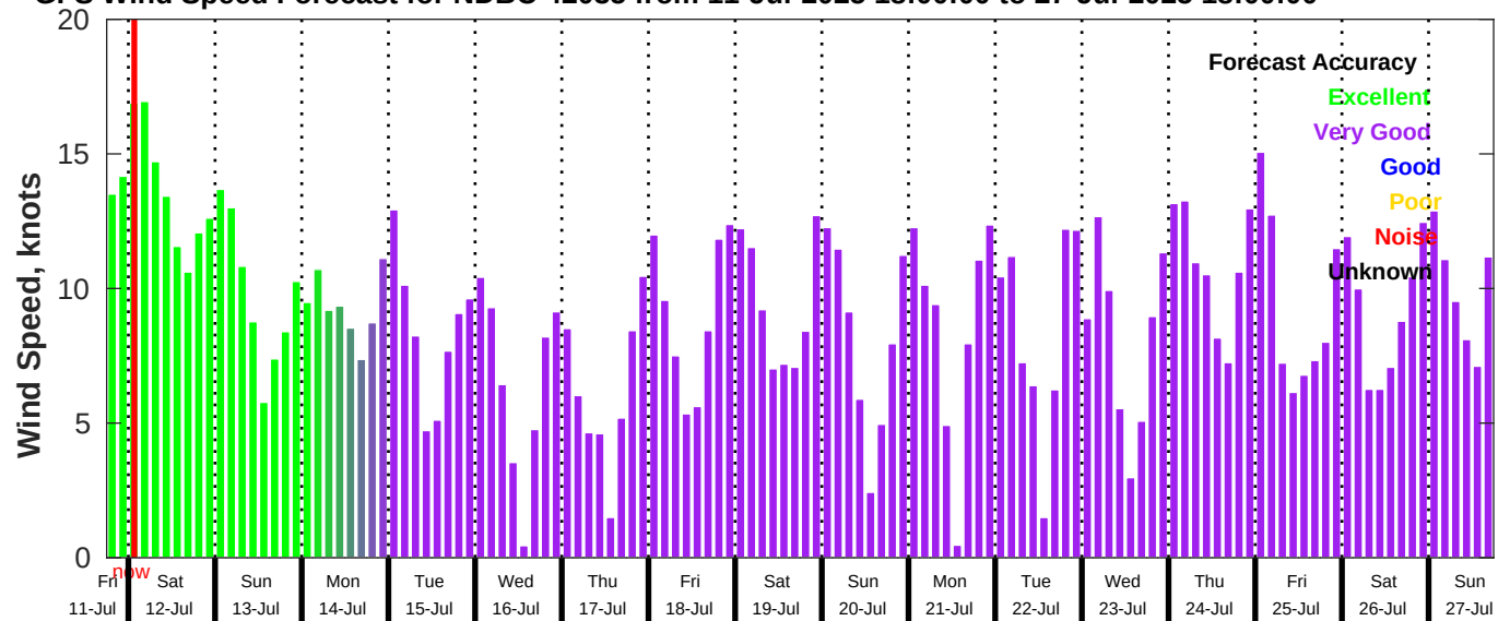
GFS Wind Speed Forecast for NDBC 42035 from 11-Jul-2025 18:00:00 to 27-Jul-2025 18:00:00
