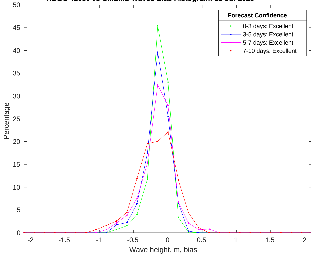
NDBC 42036 vs CMEMS Waves Bias Histogram: 12-Jul-2025
