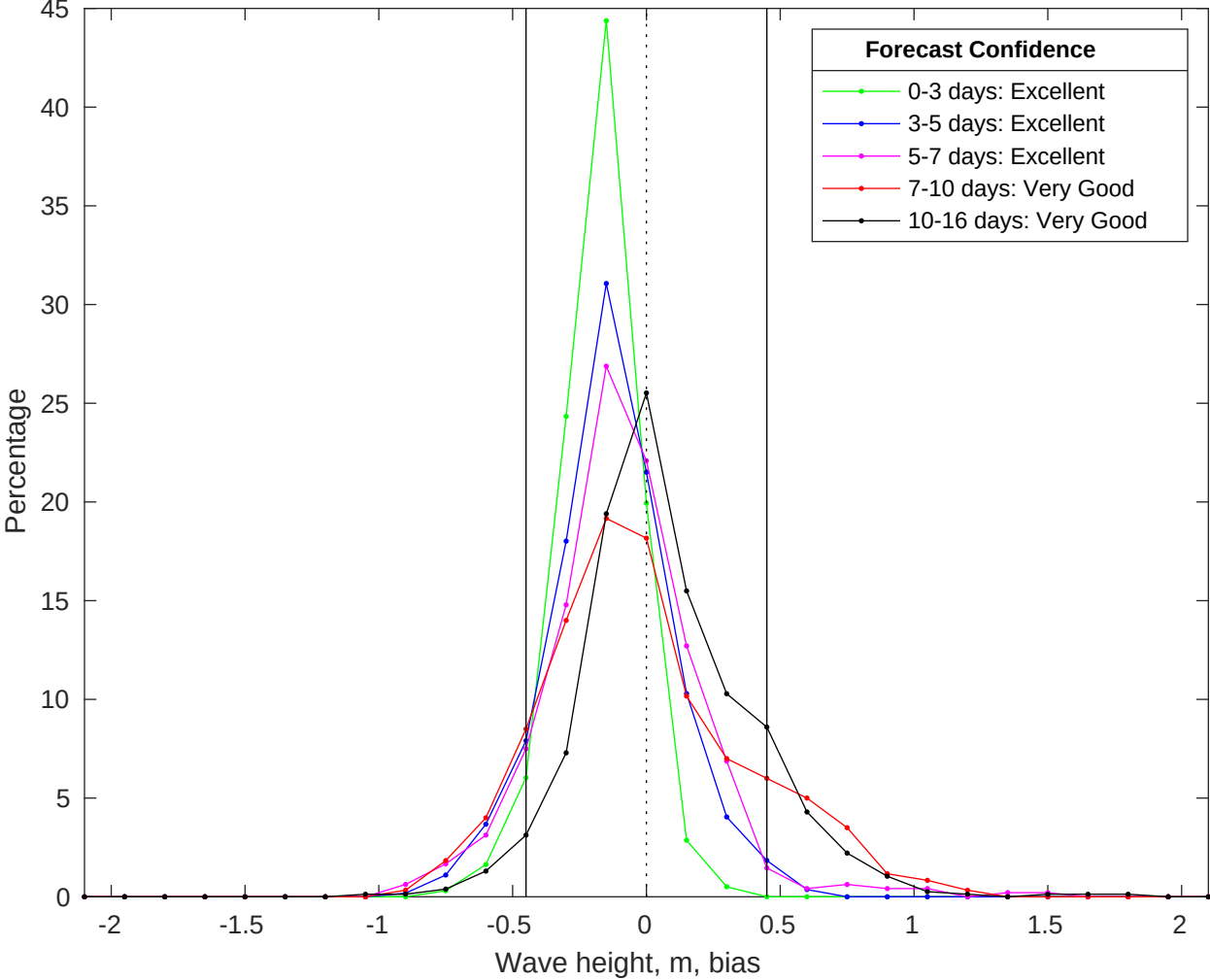
NDBC 42036 vs GFS Waves Bias Histogram: 12-Jul-2025
