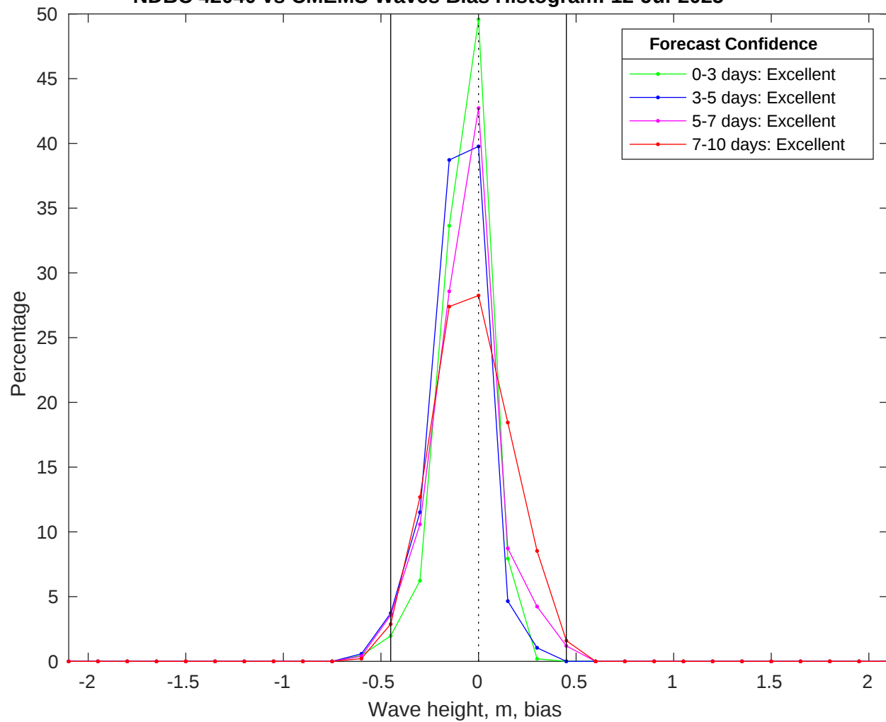
NDBC 42040 vs CMEMS Waves Bias Histogram: 12-Jul-2025
