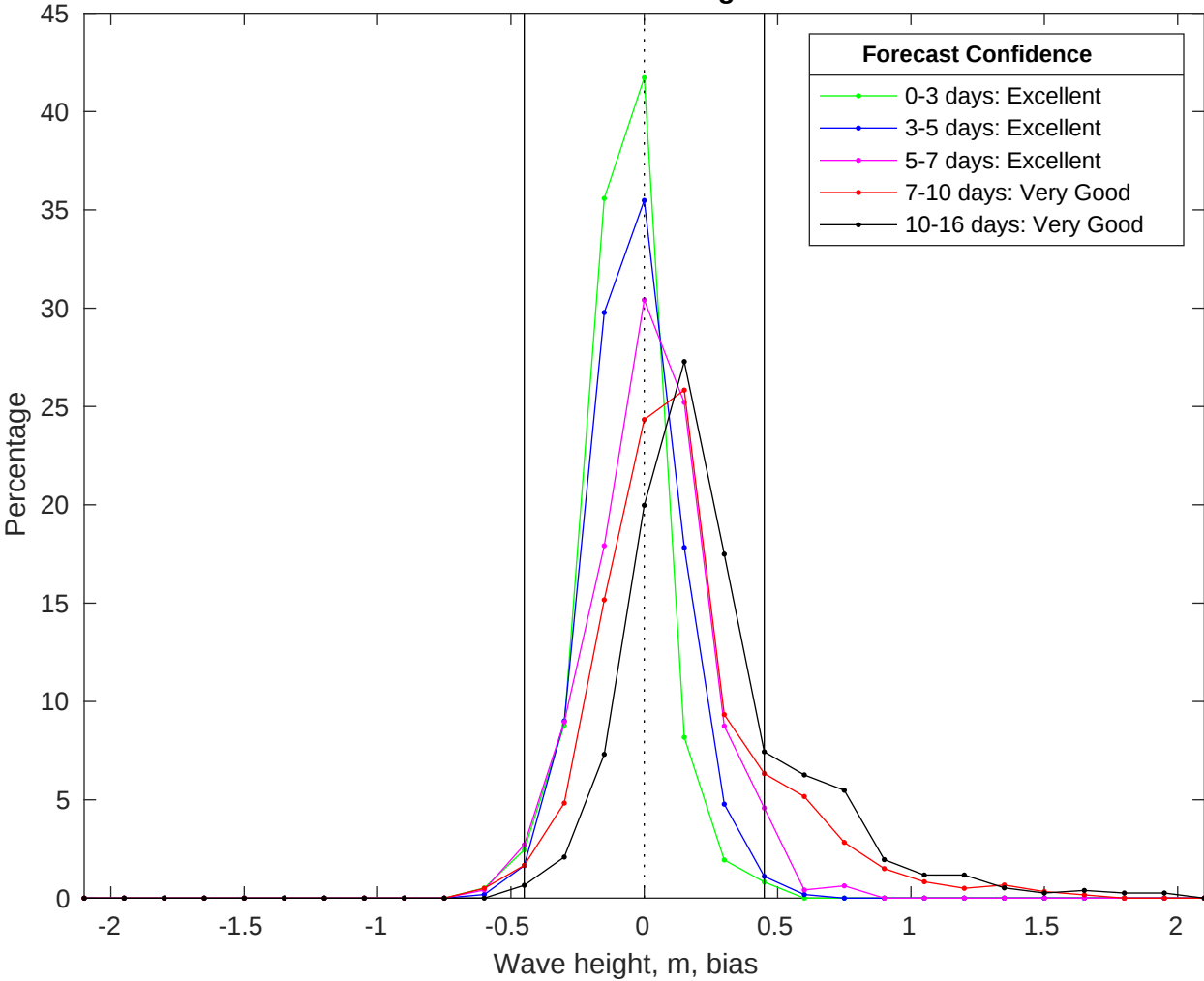
NDBC 42040 vs GFS Waves Bias Histogram: 12-Jul-2025
