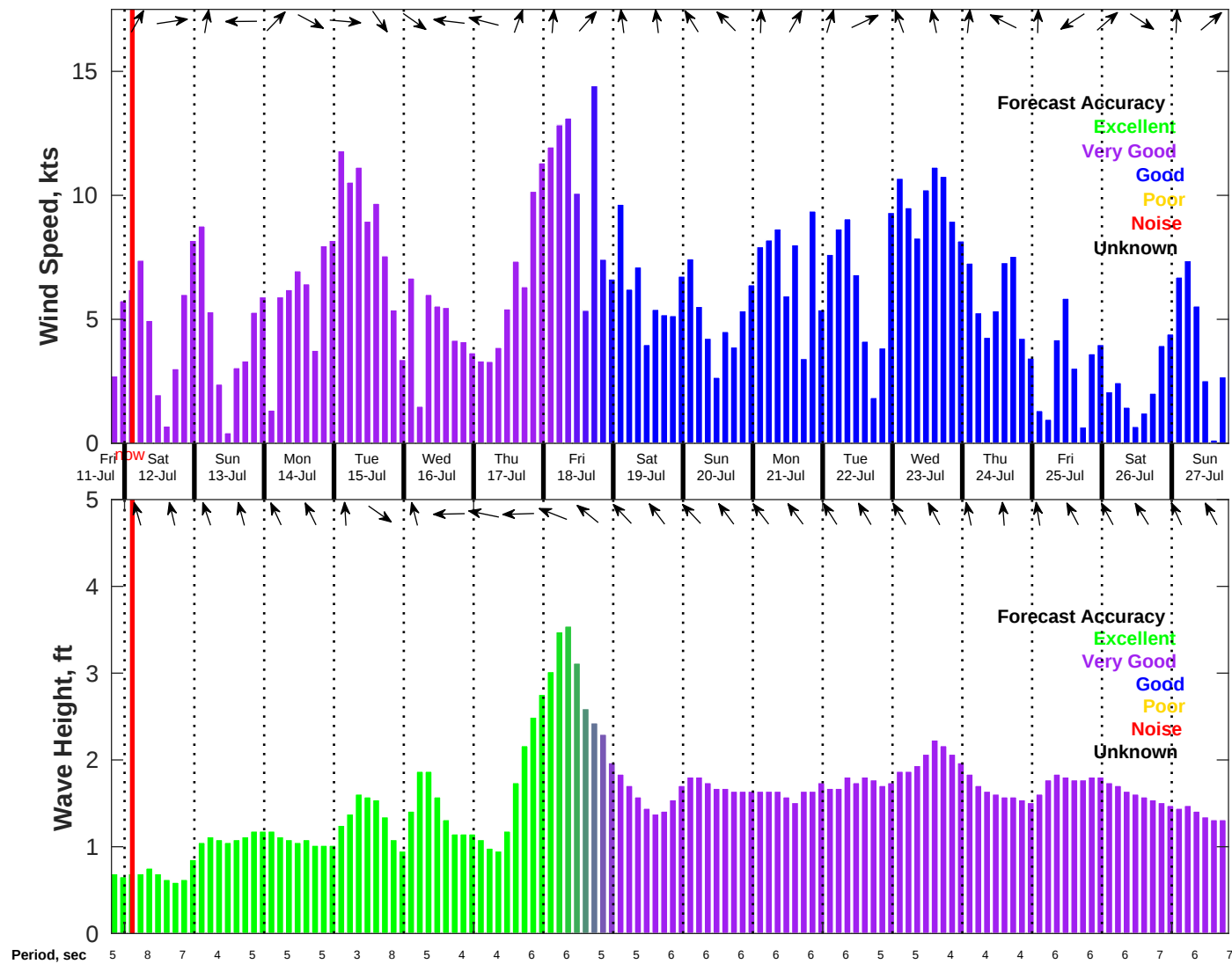
Wind & Wave Forecast for NDBC 42040 from 11-Jul-2025 19:00:00 to 27-Jul-2025 19:00:00
