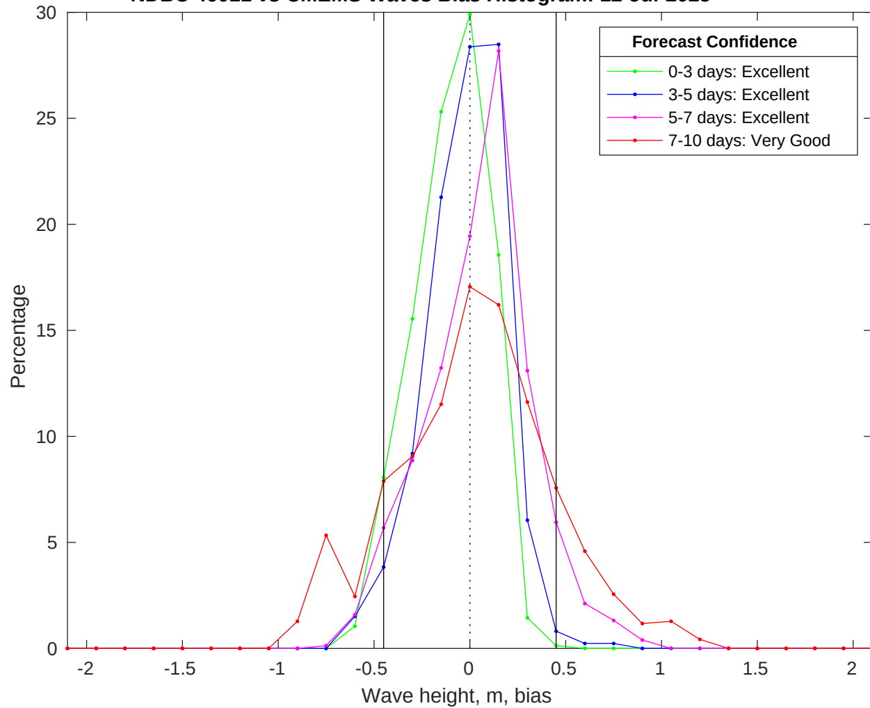
NDBC 46011 vs CMEMS Waves Bias Histogram: 12-Jul-2025
