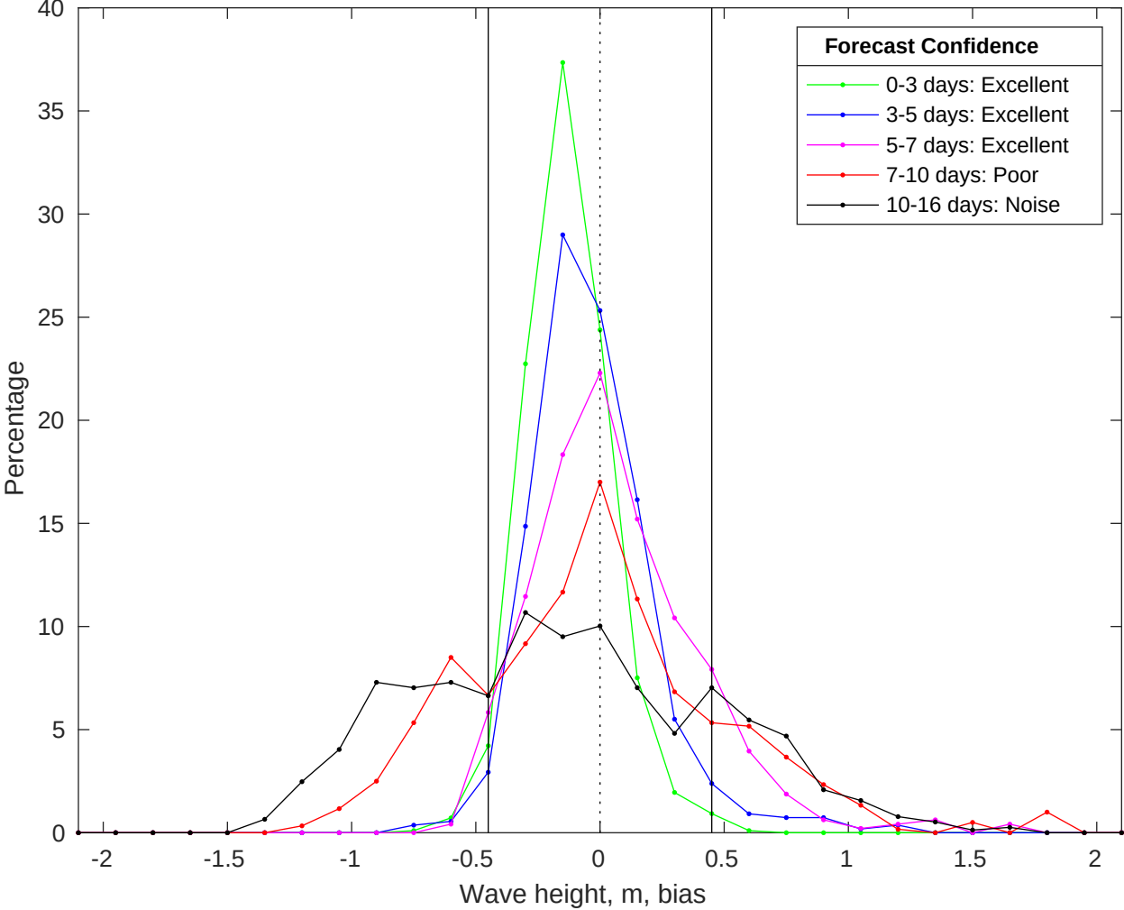
NDBC 46011 vs GFS Waves Bias Histogram: 12-Jul-2025
