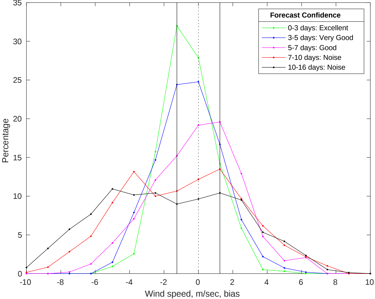
NDBC 46011 vs GFS Winds Bias Histogram: 12-Jul-2025
