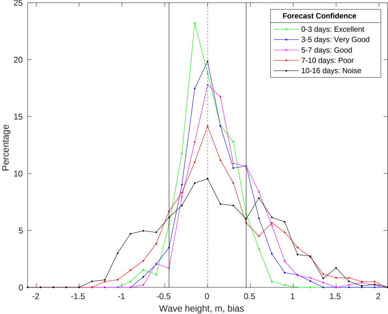
NDBC 46028 vs GFS Waves Bias Histogram: 12-Jul-2025
