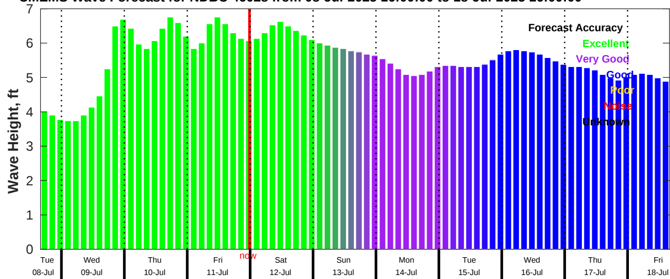
CMEMS Wave Forecast for NDBC 46028 from 08-Jul-2025 16:00:00 to 18-Jul-2025 16:00:00
