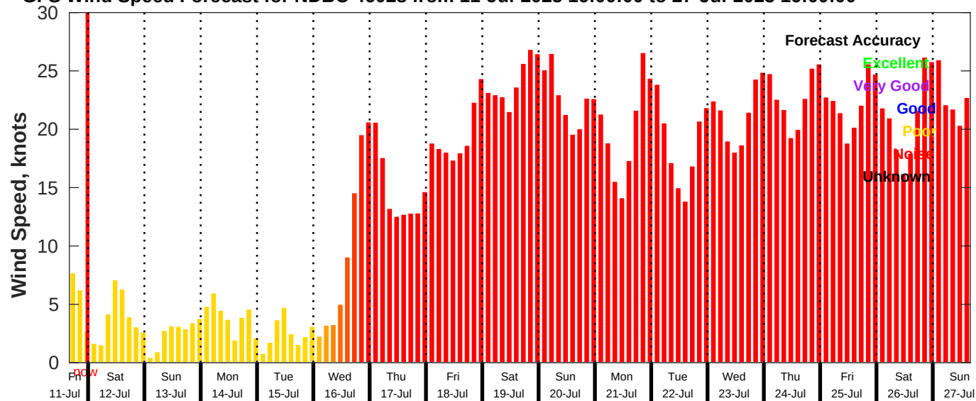
GFS Wind Speed Forecast for NDBC 46028 from 11-Jul-2025 16:00:00 to 27-Jul-2025 16:00:00
