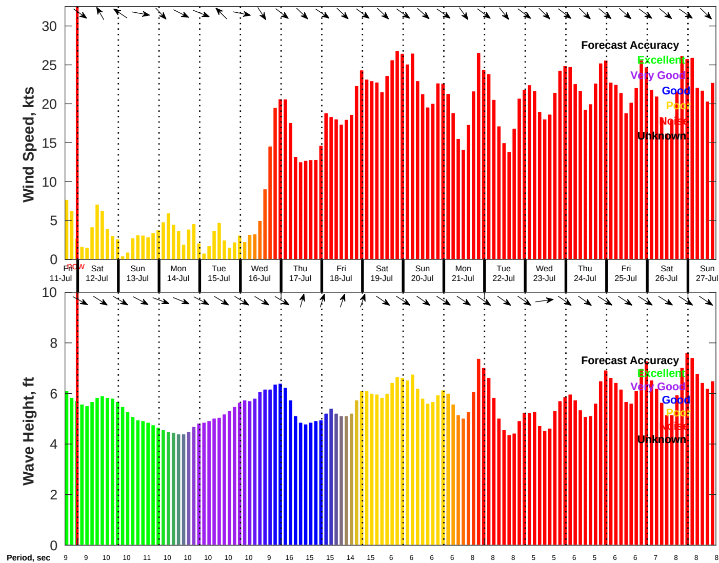
Wind & Wave Forecast for NDBC 46028 from 11-Jul-2025 16:00:00 to 27-Jul-2025 16:00:00
