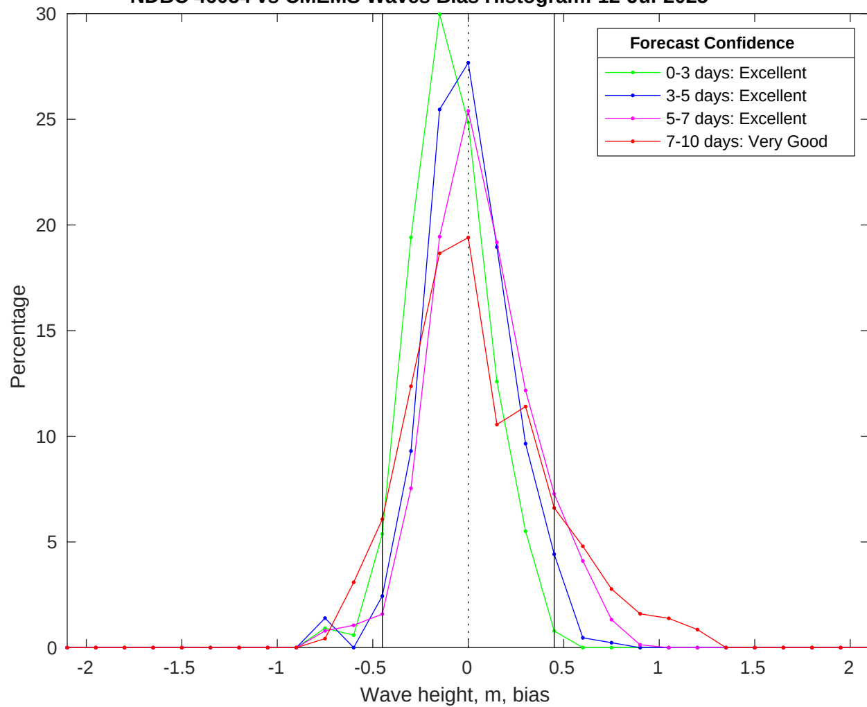
NDBC 46054 vs CMEMS Waves Bias Histogram: 12-Jul-2025
