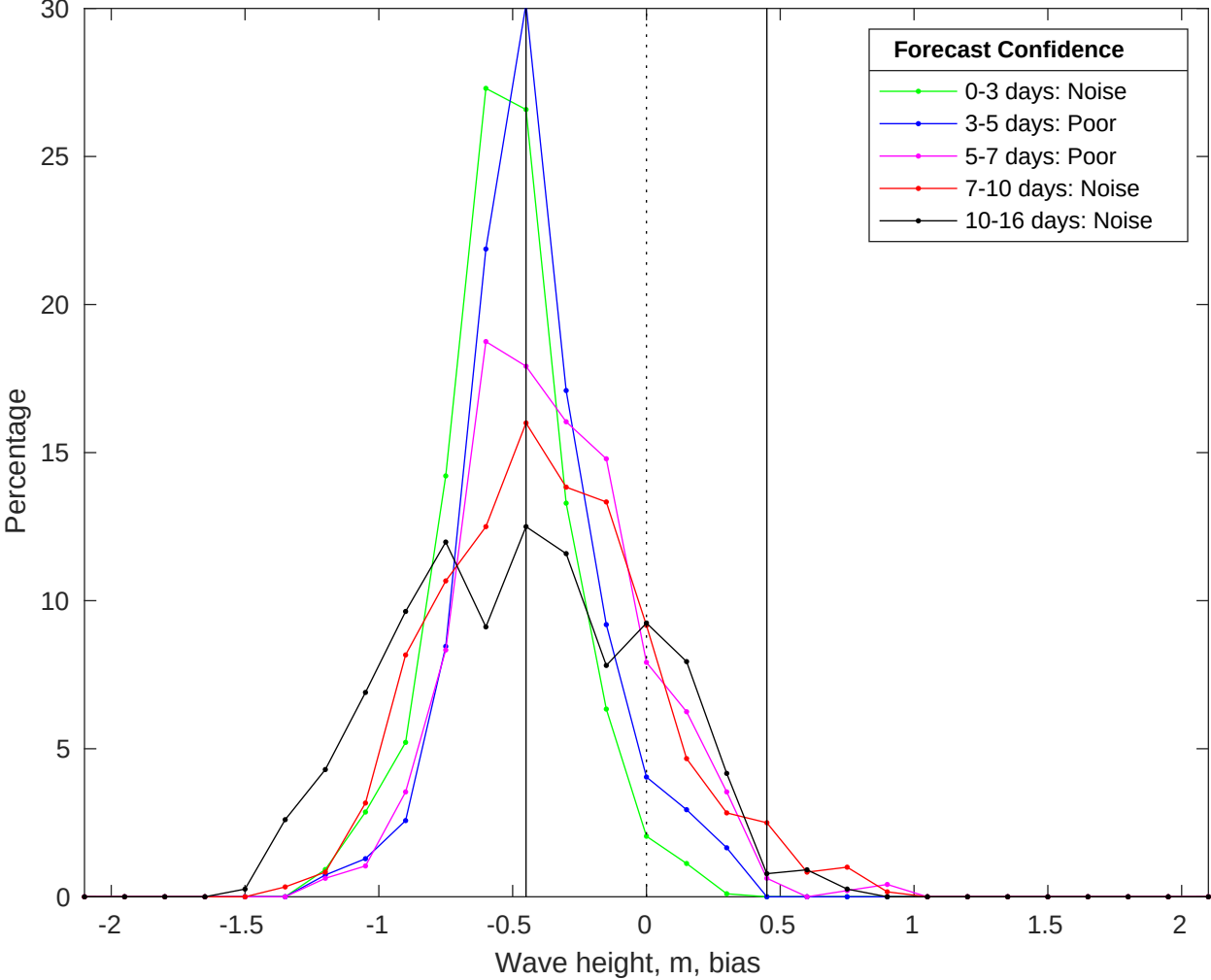
NDBC 46054 vs GFS Waves Bias Histogram: 12-Jul-2025
