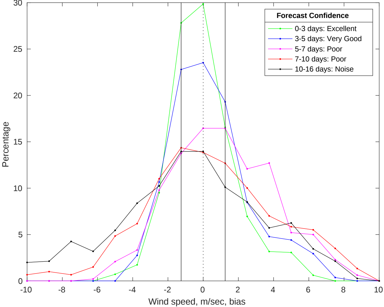
NDBC 46054 vs GFS Winds Bias Histogram: 12-Jul-2025
