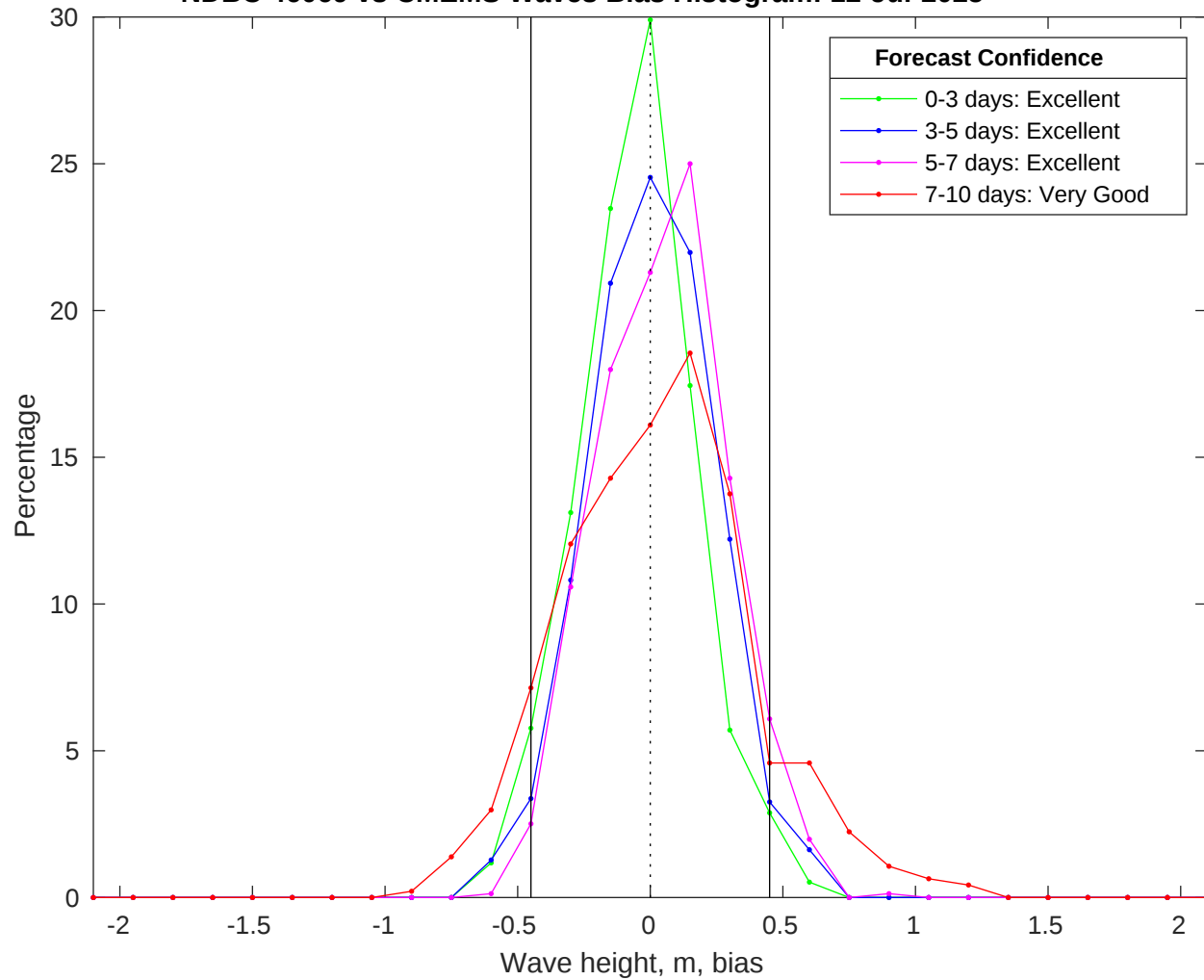
NDBC 46069 vs CMEMS Waves Bias Histogram: 12-Jul-2025
