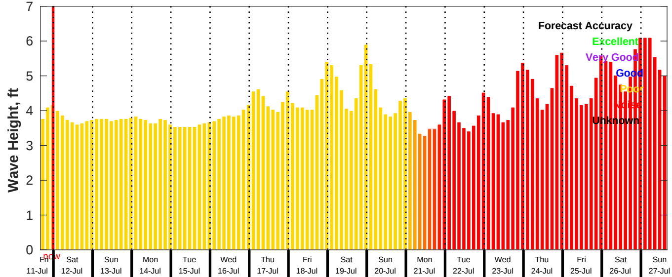
GFS Wave Forecast for NDBC 46069 from 11-Jul-2025 16:00:00 to 27-Jul-2025 16:00:00
