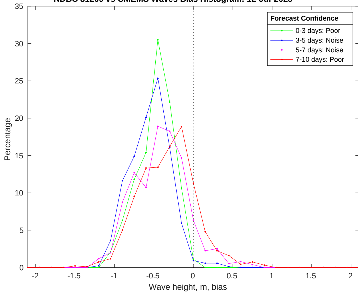
NDBC 51209 vs CMEMS Waves Bias Histogram: 12-Jul-2025
