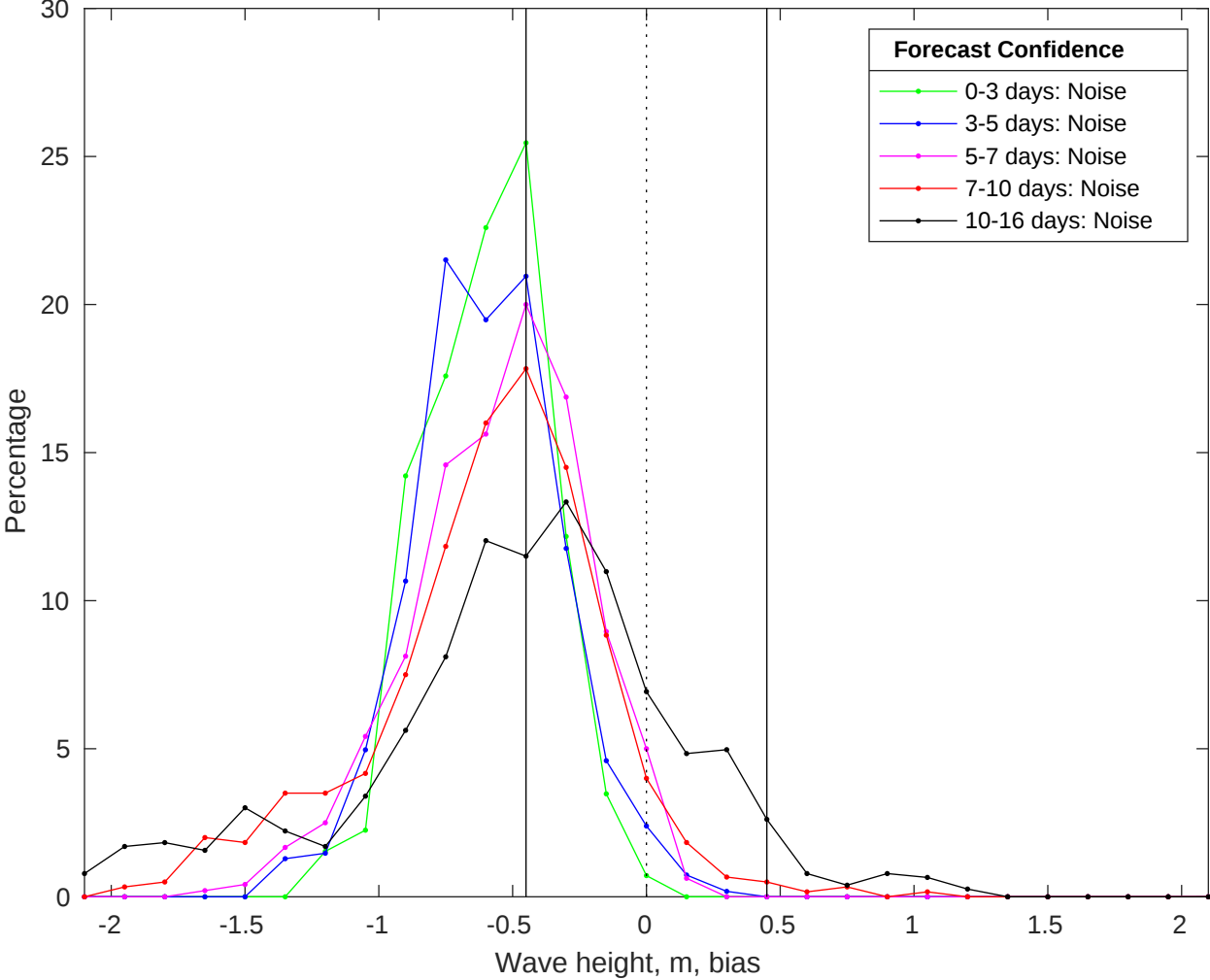
NDBC 51209 vs GFS Waves Bias Histogram: 12-Jul-2025
