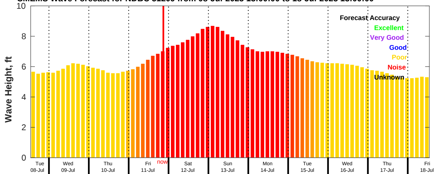
CMEMS Wave Forecast for NDBC 51209 from 08-Jul-2025 13:00:00 to 18-Jul-2025 13:00:00
