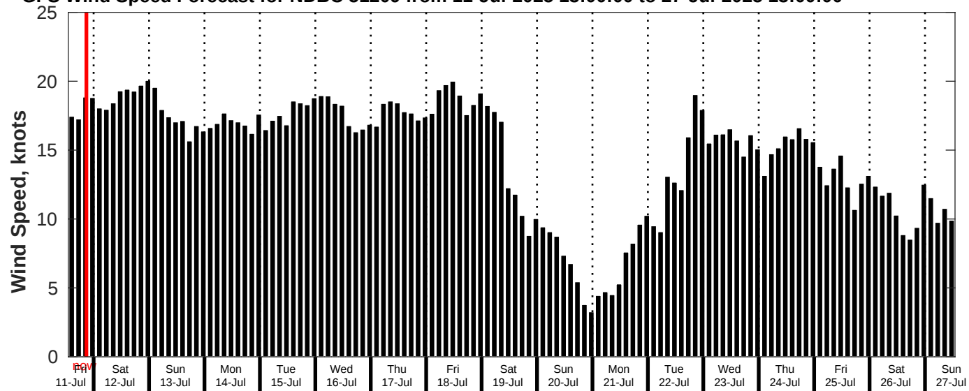
GFS Wind Speed Forecast for NDBC 51209 from 11-Jul-2025 13:00:00 to 27-Jul-2025 13:00:00
