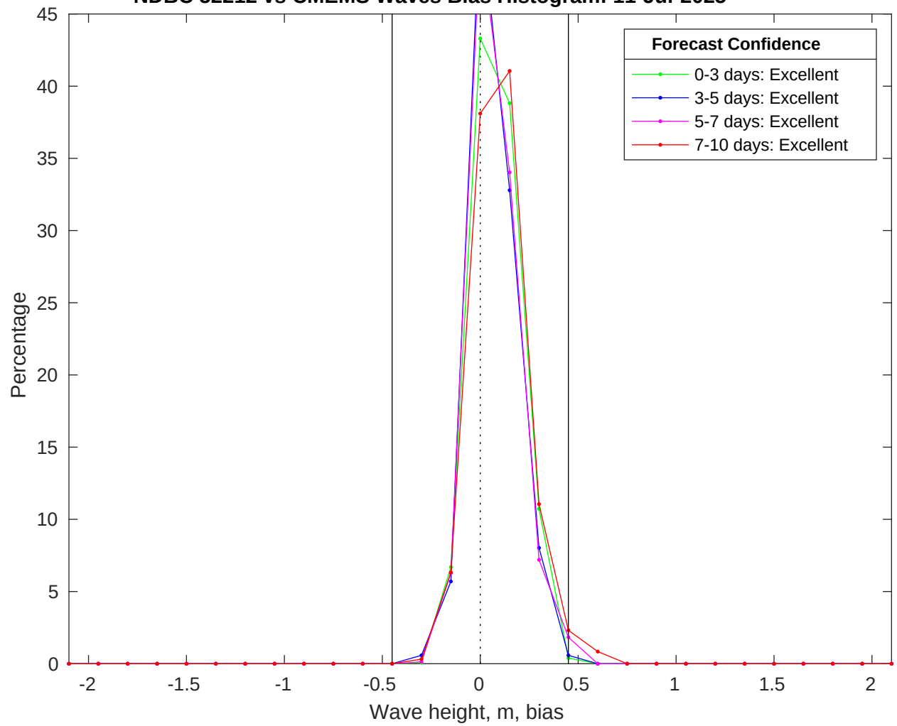
NDBC 52212 vs CMEMS Waves Bias Histogram: 11-Jul-2025
