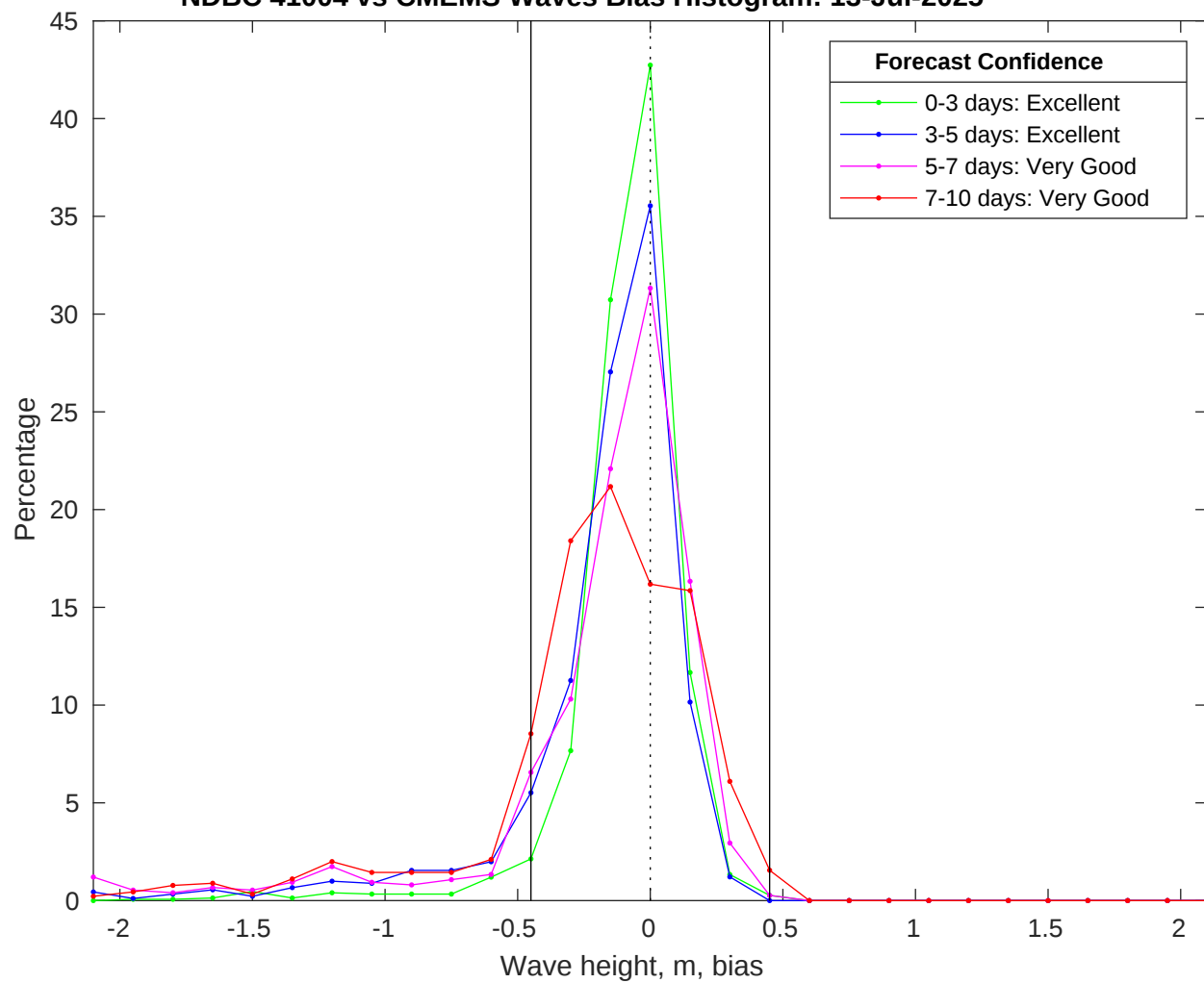
NDBC 41004 vs CMEMS Waves Bias Histogram: 13-Jul-2025
