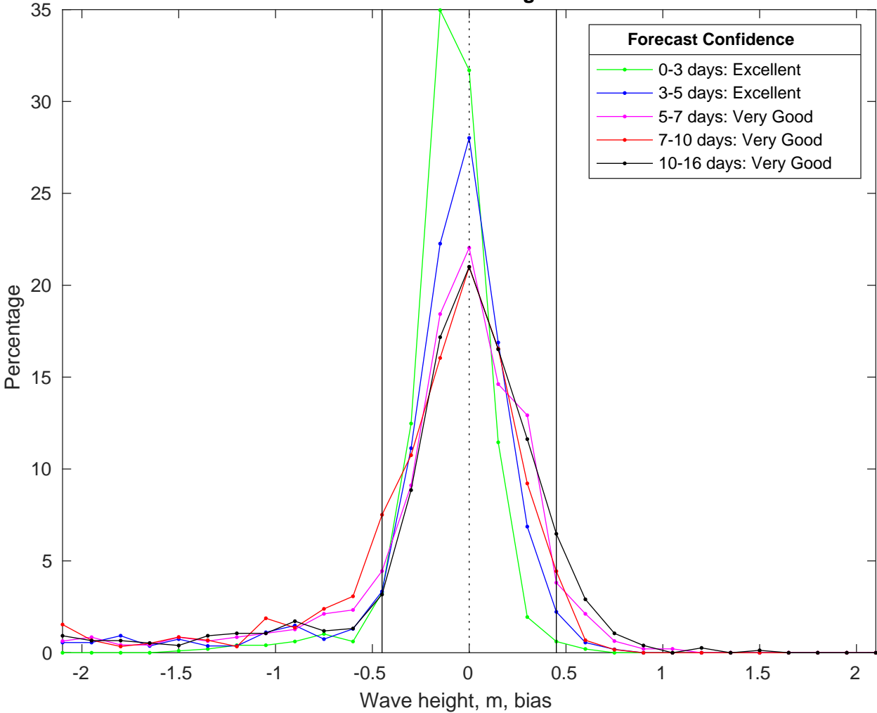
NDBC 41004 vs GFS Waves Bias Histogram: 13-Jul-2025
