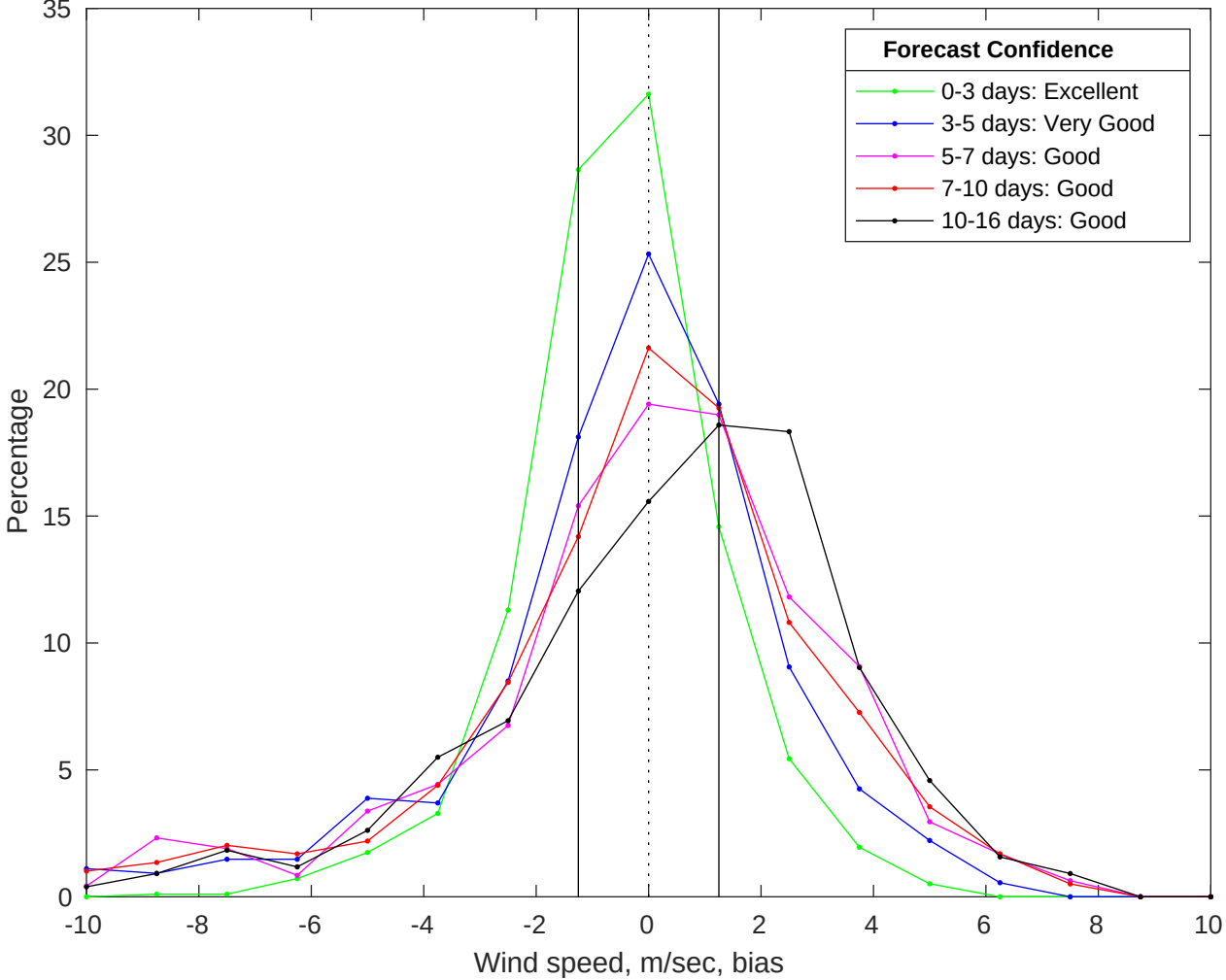
NDBC 41004 vs GFS Winds Bias Histogram: 13-Jul-2025
