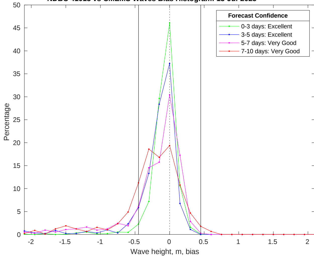
NDBC 41013 vs CMEMS Waves Bias Histogram: 13-Jul-2025
