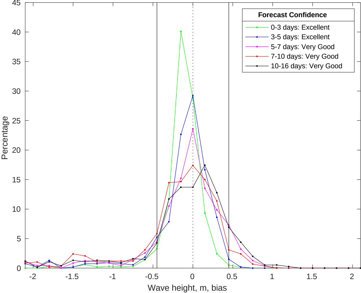
NDBC 41013 vs GFS Waves Bias Histogram: 13-Jul-2025
