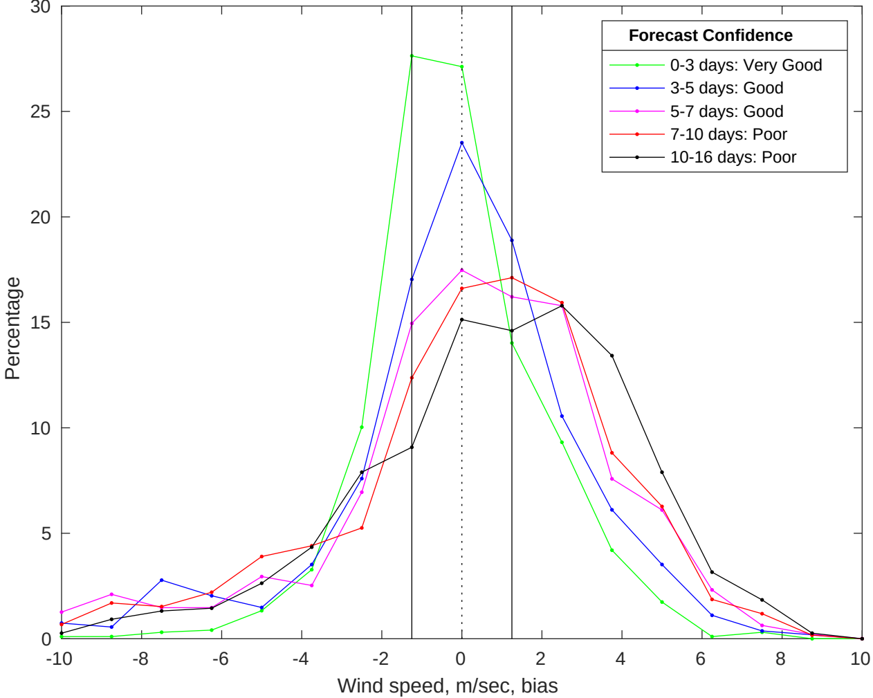
NDBC 41013 vs GFS Winds Bias Histogram: 13-Jul-2025
