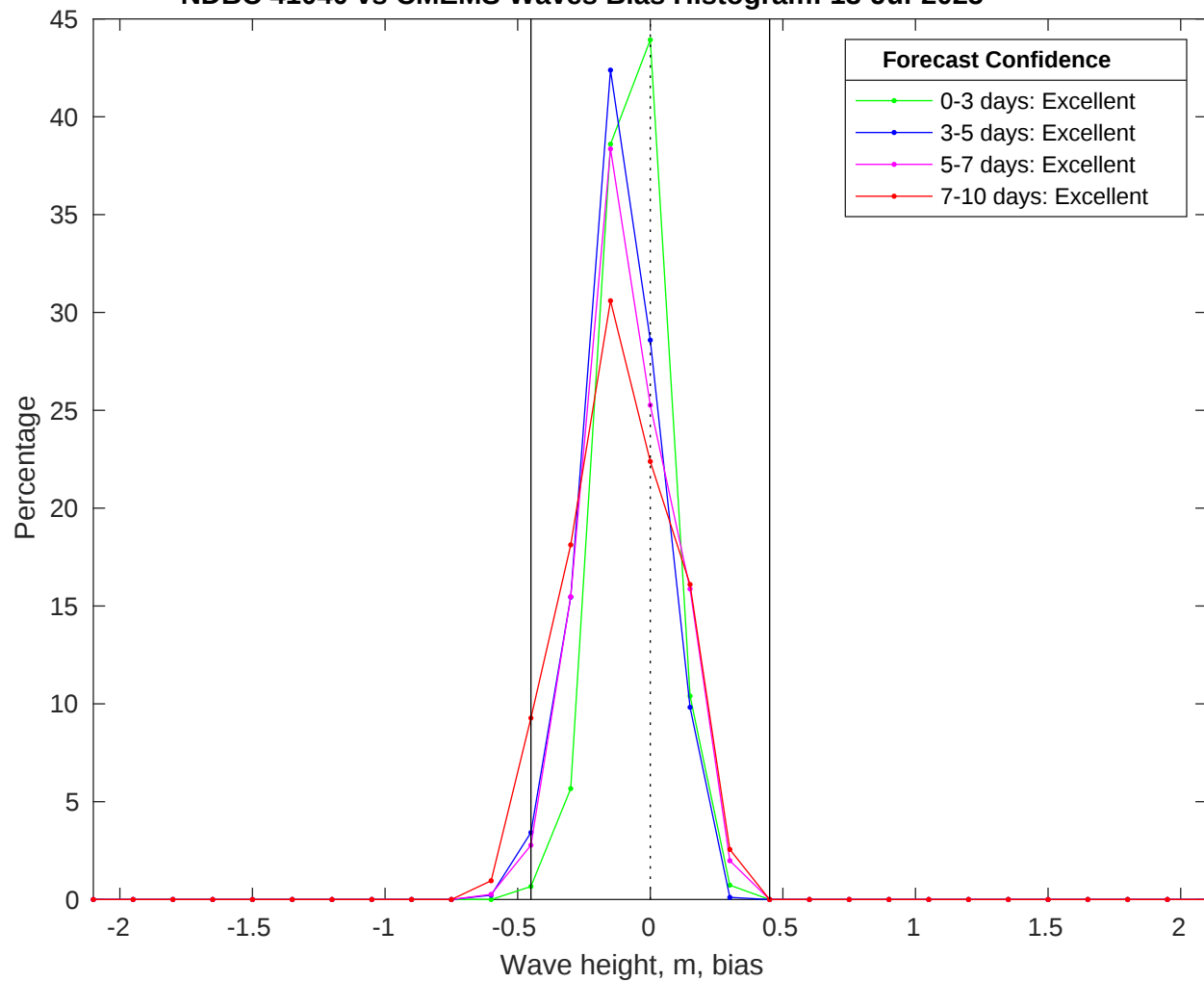
NDBC 41040 vs CMEMS Waves Bias Histogram: 13-Jul-2025
