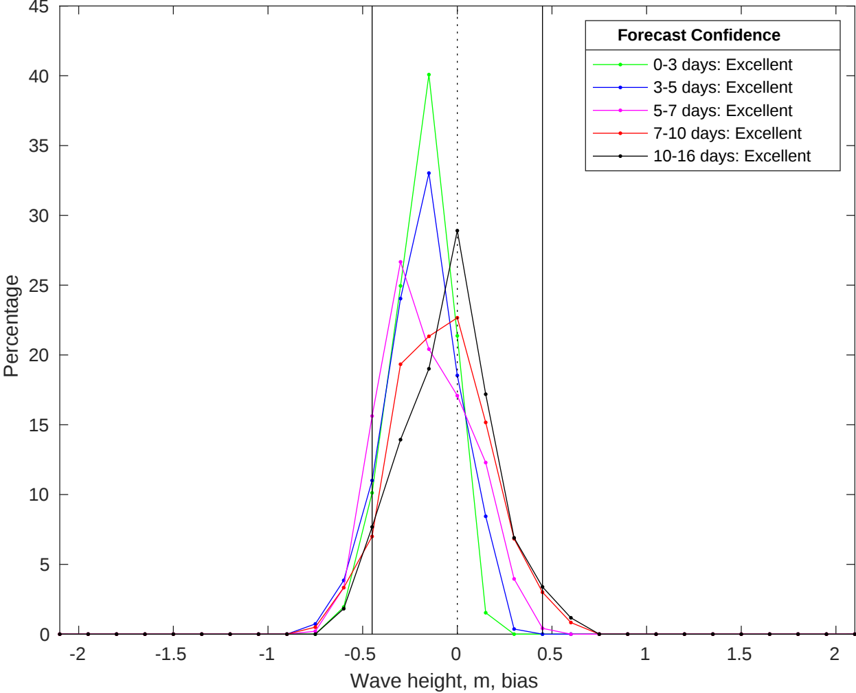
NDBC 41040 vs GFS Waves Bias Histogram: 13-Jul-2025
