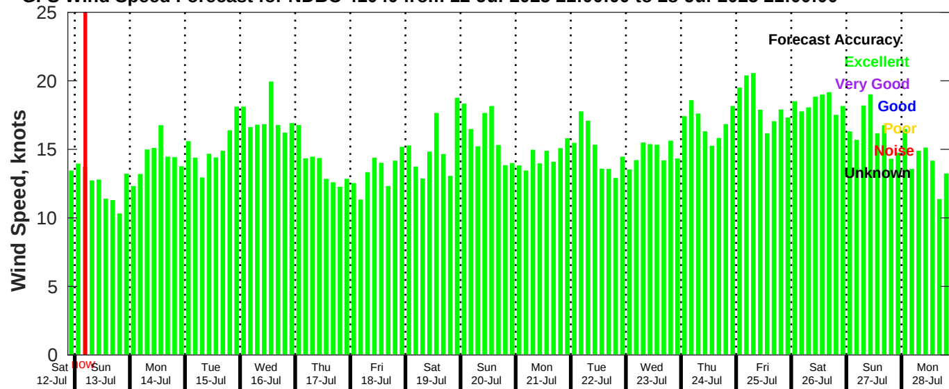
GFS Wind Speed Forecast for NDBC 41040 from 12-Jul-2025 21:00:00 to 28-Jul-2025 21:00:00
