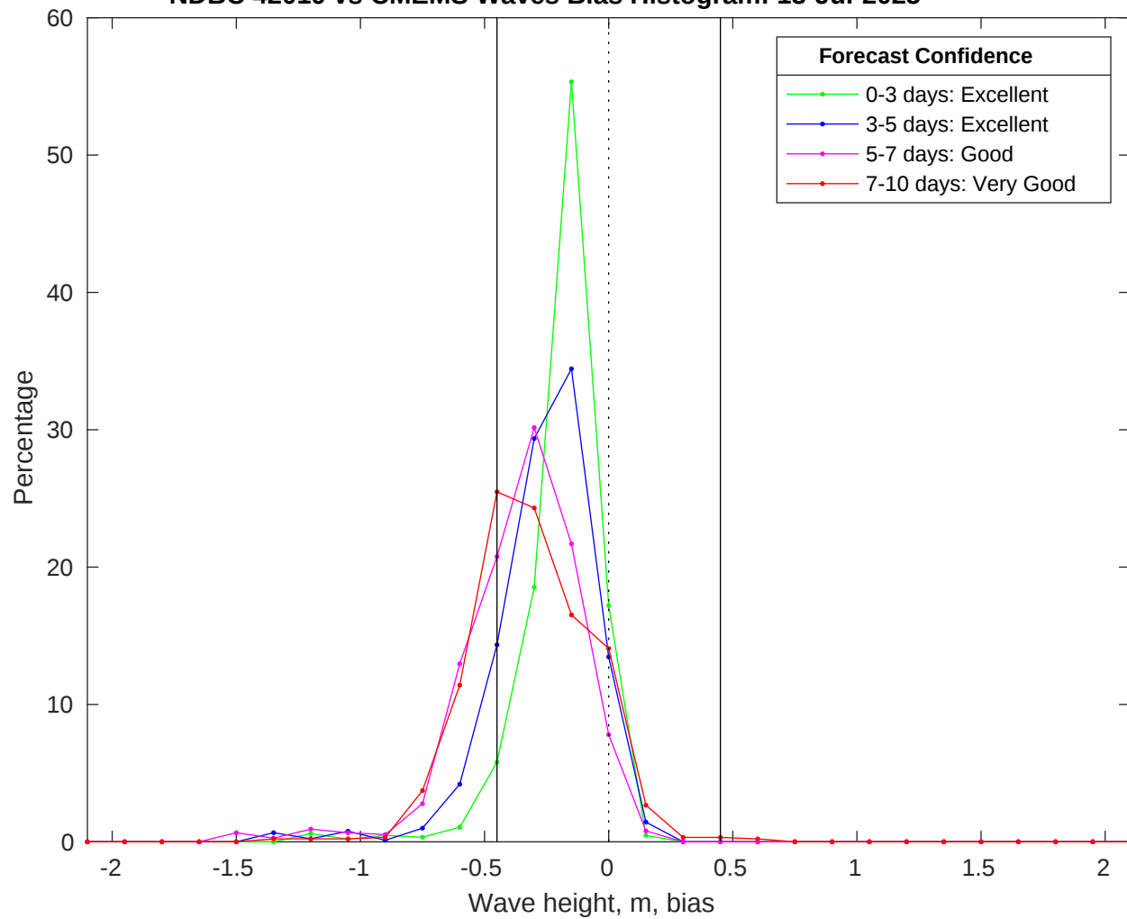
NDBC 42019 vs CMEMS Waves Bias Histogram: 13-Jul-2025
