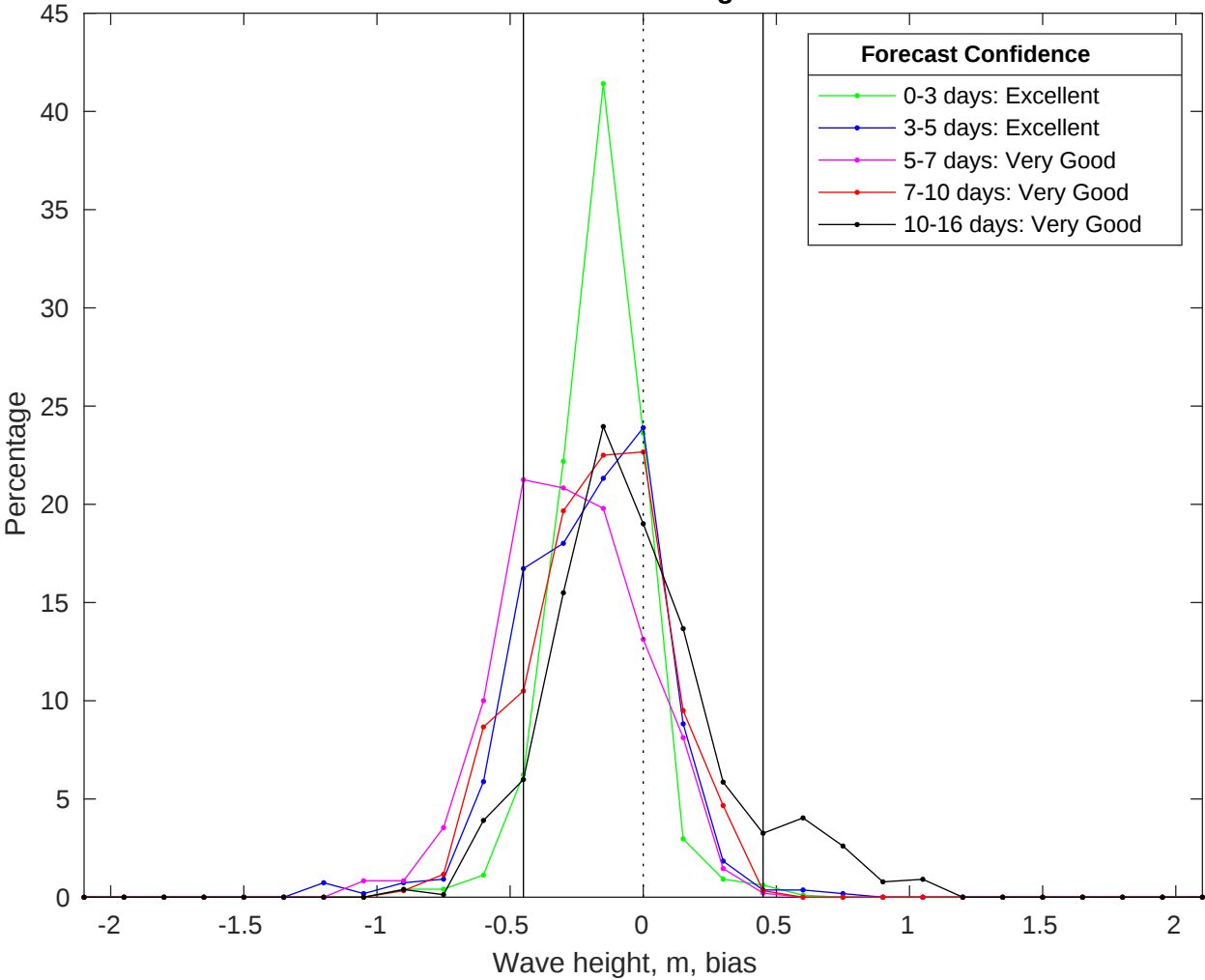
NDBC 42019 vs GFS Waves Bias Histogram: 13-Jul-2025
