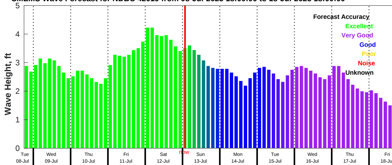
CMEMS Wave Forecast for NDBC 42019 from 08-Jul-2025 18:00:00 to 18-Jul-2025 18:00:00
