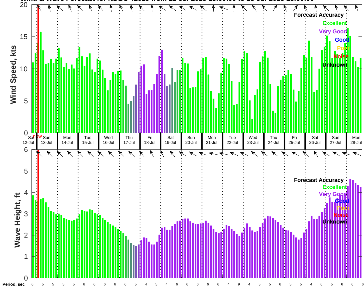
Wind & Wave Forecast for NDBC 42019 from 12-Jul-2025 18:00:00 to 28-Jul-2025 18:00:00
