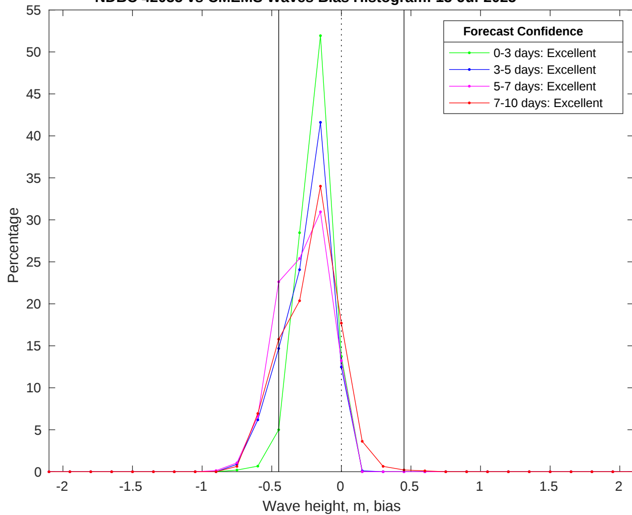
NDBC 42035 vs CMEMS Waves Bias Histogram: 13-Jul-2025
