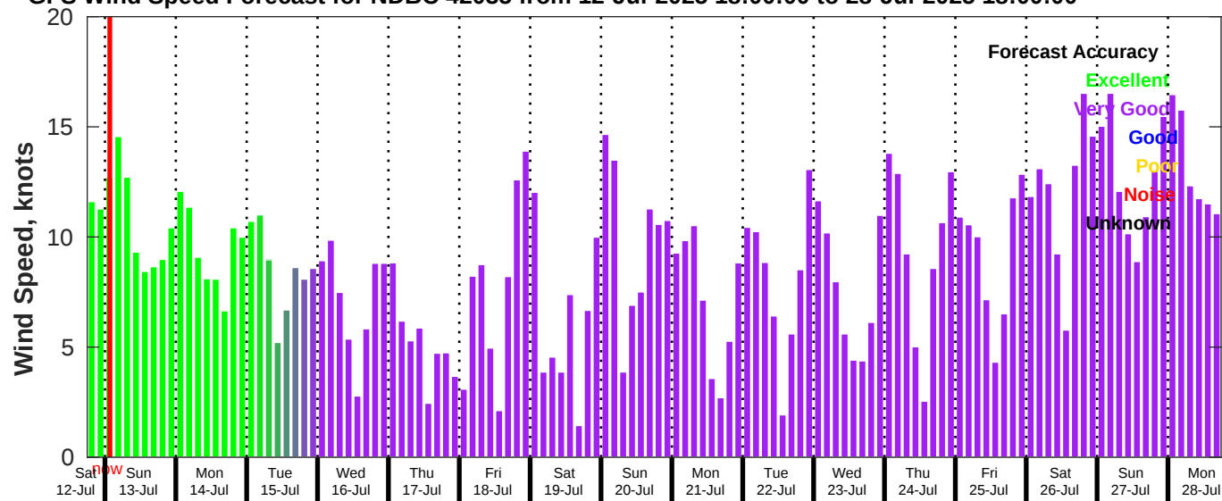
GFS Wind Speed Forecast for NDBC 42035 from 12-Jul-2025 18:00:00 to 28-Jul-2025 18:00:00
