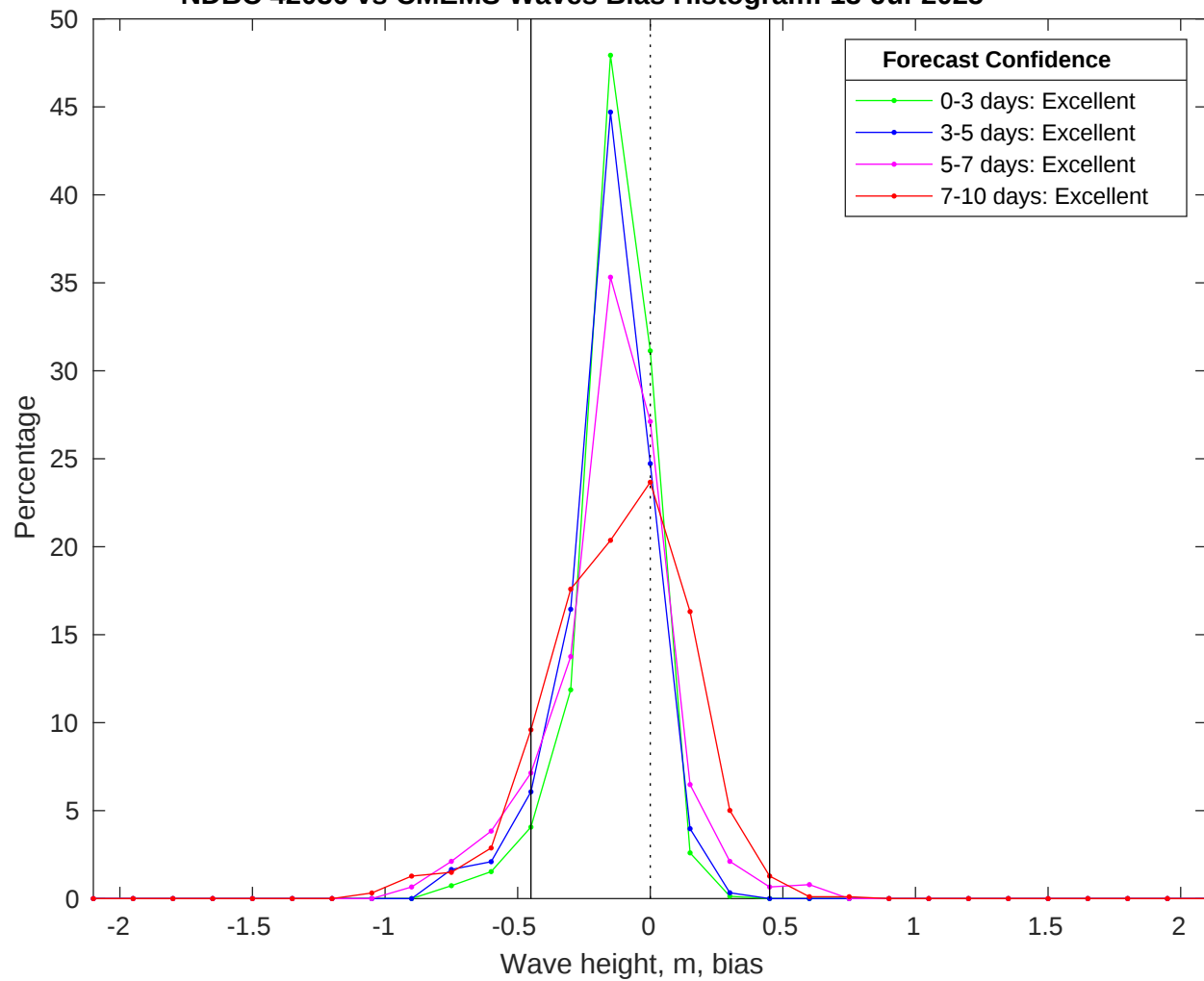
NDBC 42036 vs CMEMS Waves Bias Histogram: 13-Jul-2025
