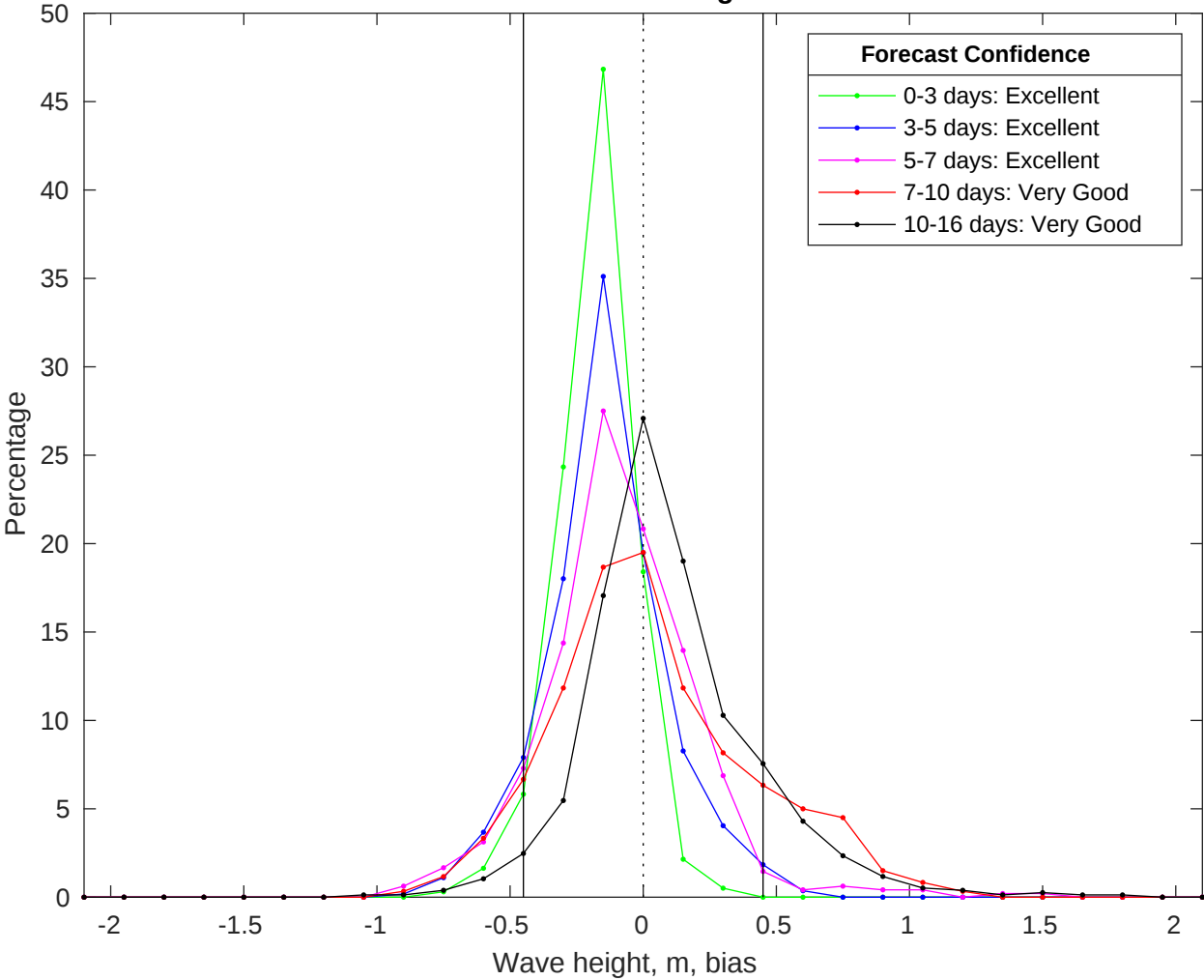
NDBC 42036 vs GFS Waves Bias Histogram: 13-Jul-2025
