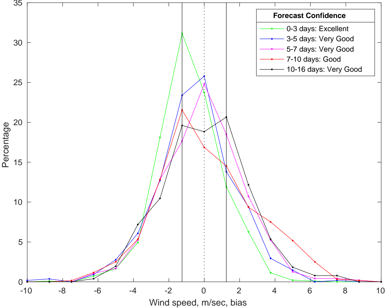
NDBC 42036 vs GFS Winds Bias Histogram: 13-Jul-2025
