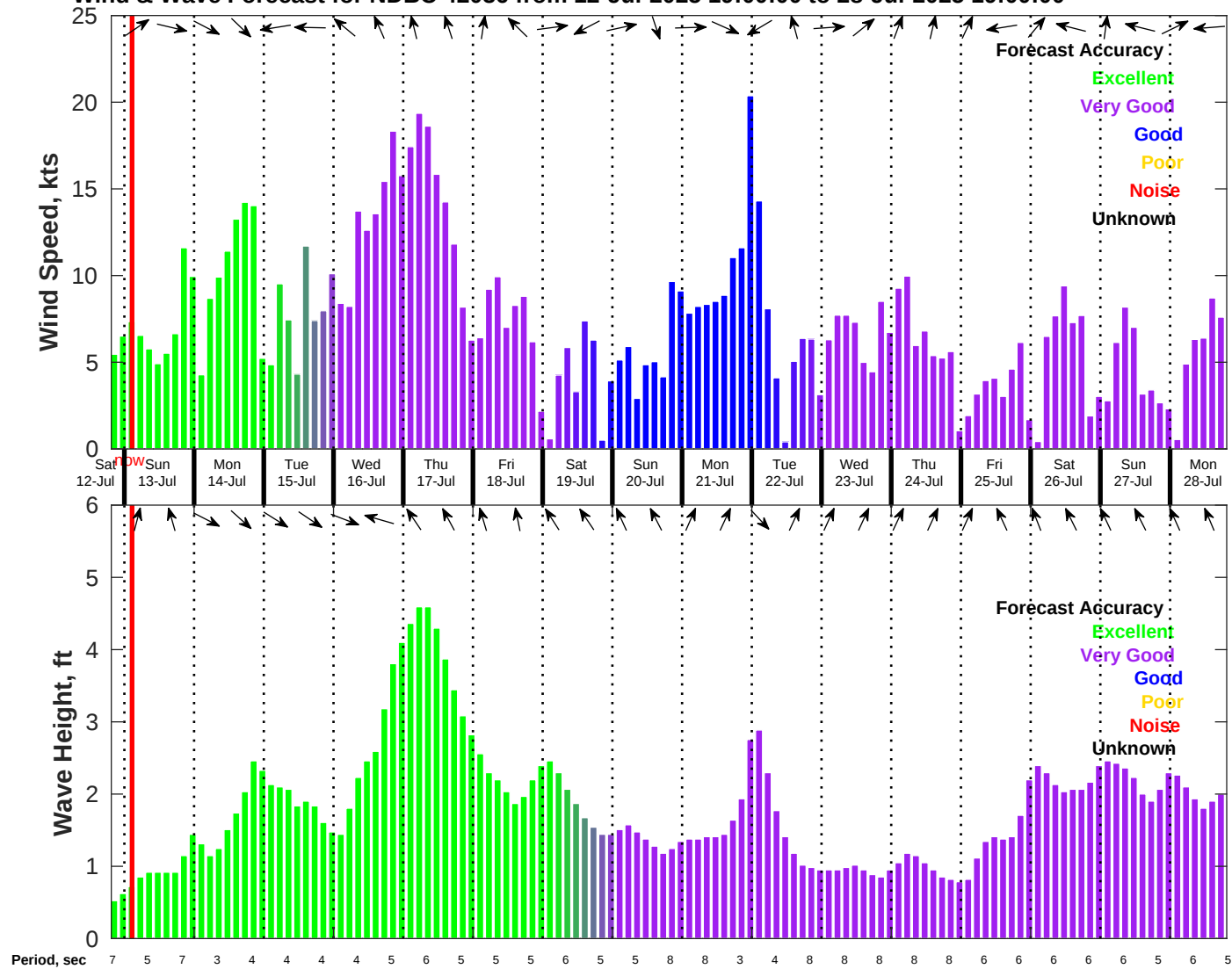
Wind & Wave Forecast for NDBC 42036 from 12-Jul-2025 19:00:00 to 28-Jul-2025 19:00:00
