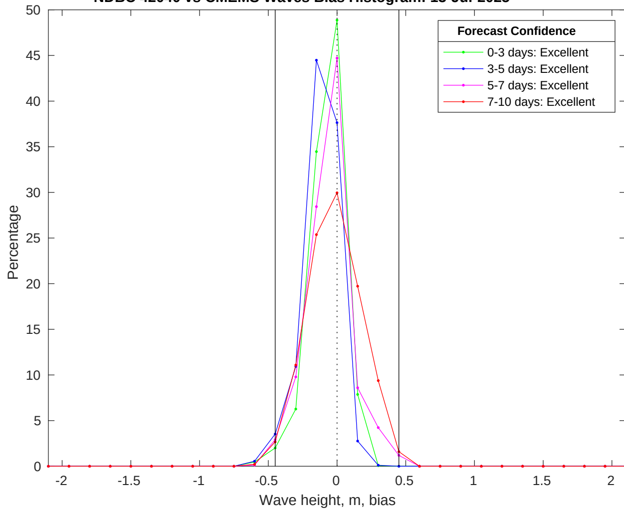
NDBC 42040 vs CMEMS Waves Bias Histogram: 13-Jul-2025
