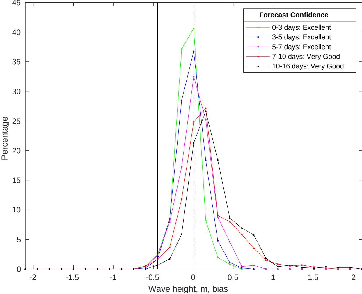
NDBC 42040 vs GFS Waves Bias Histogram: 13-Jul-2025
