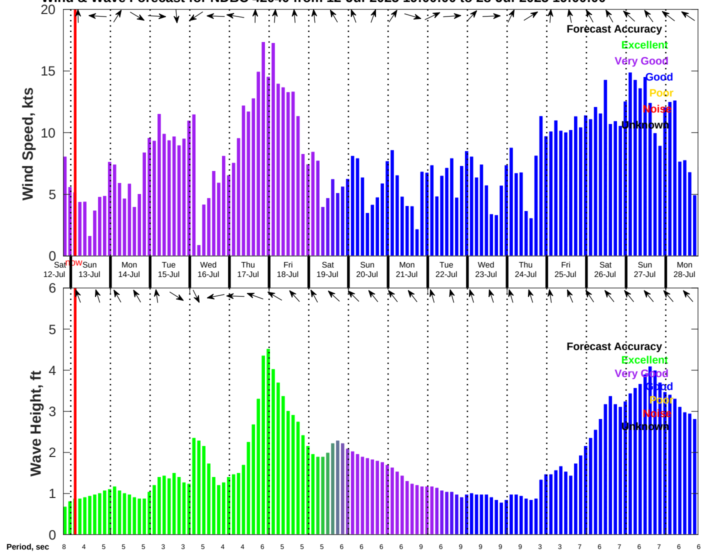
Wind & Wave Forecast for NDBC 42040 from 12-Jul-2025 19:00:00 to 28-Jul-2025 19:00:00
