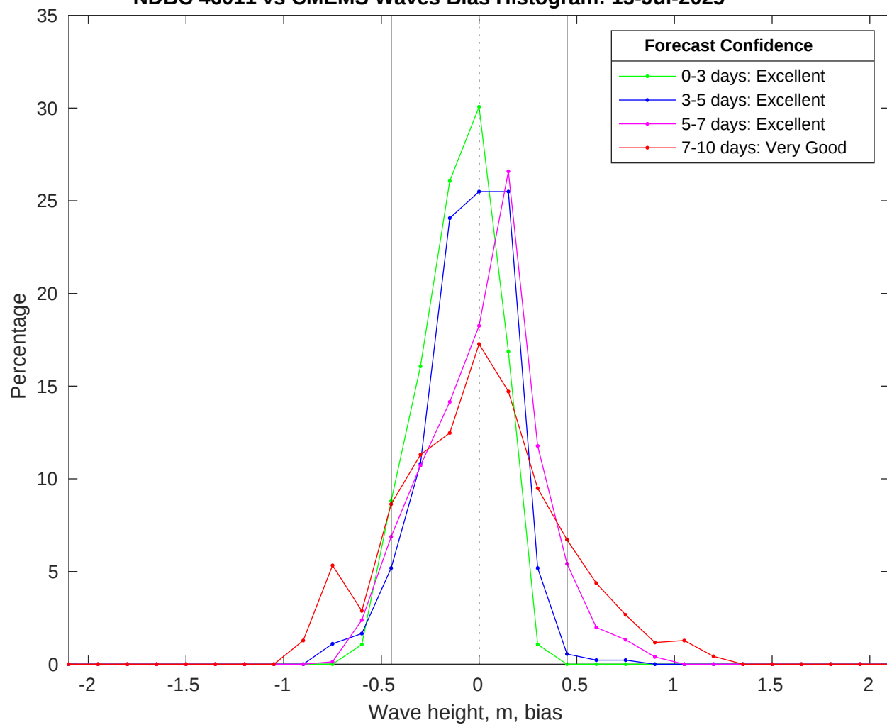
NDBC 46011 vs CMEMS Waves Bias Histogram: 13-Jul-2025
