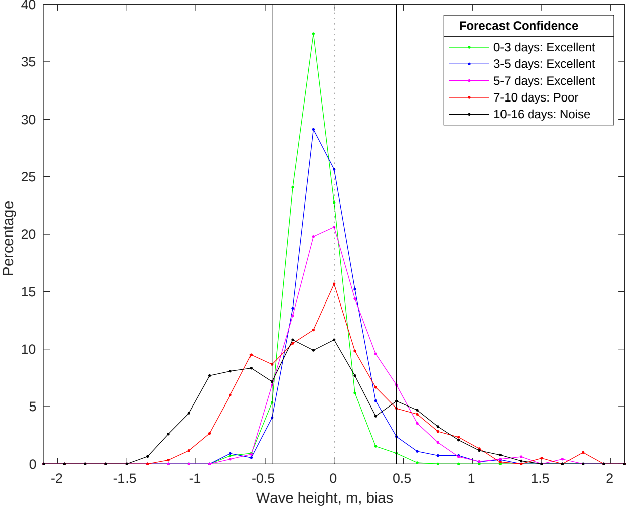
NDBC 46011 vs GFS Waves Bias Histogram: 13-Jul-2025
