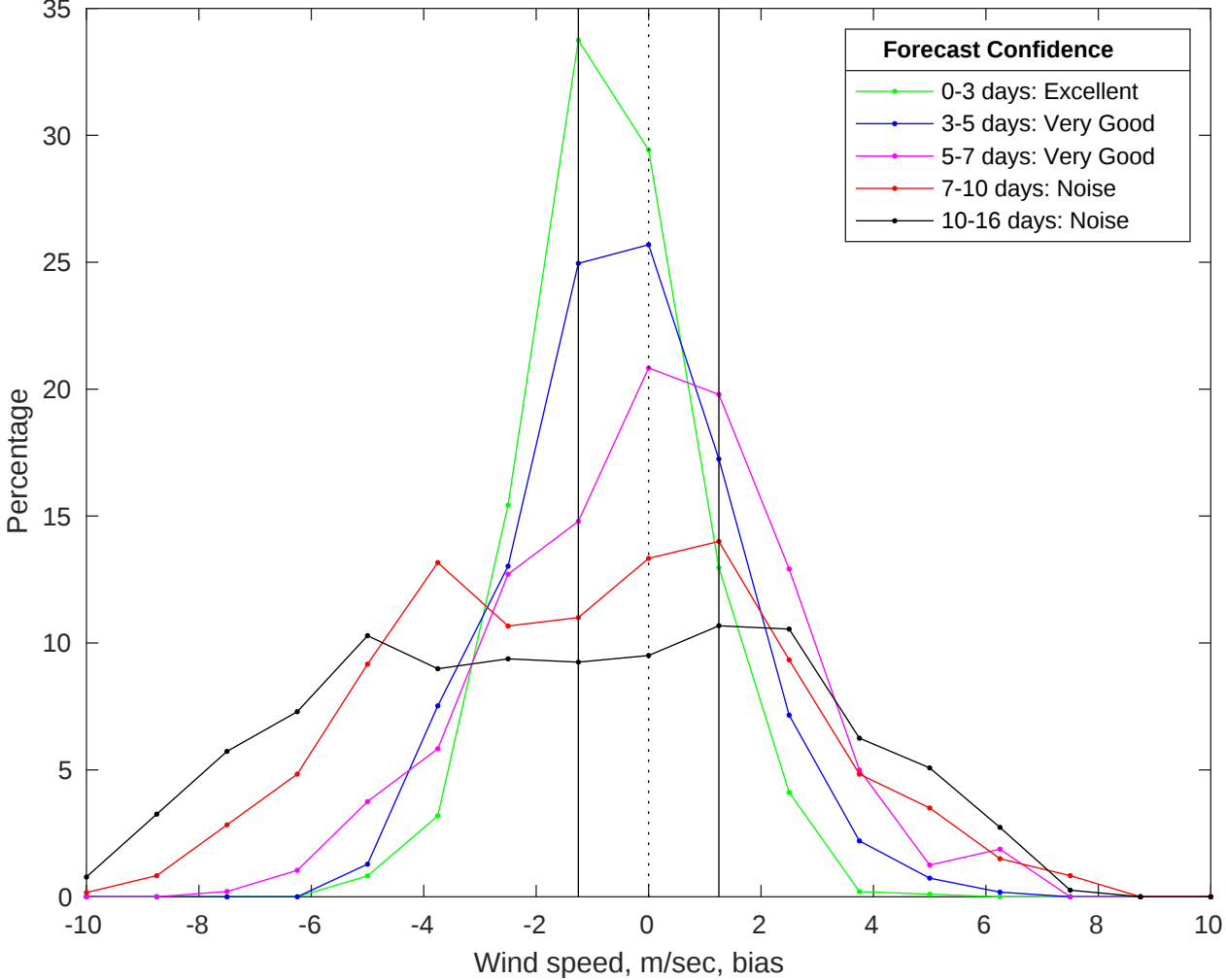
NDBC 46011 vs GFS Winds Bias Histogram: 13-Jul-2025
