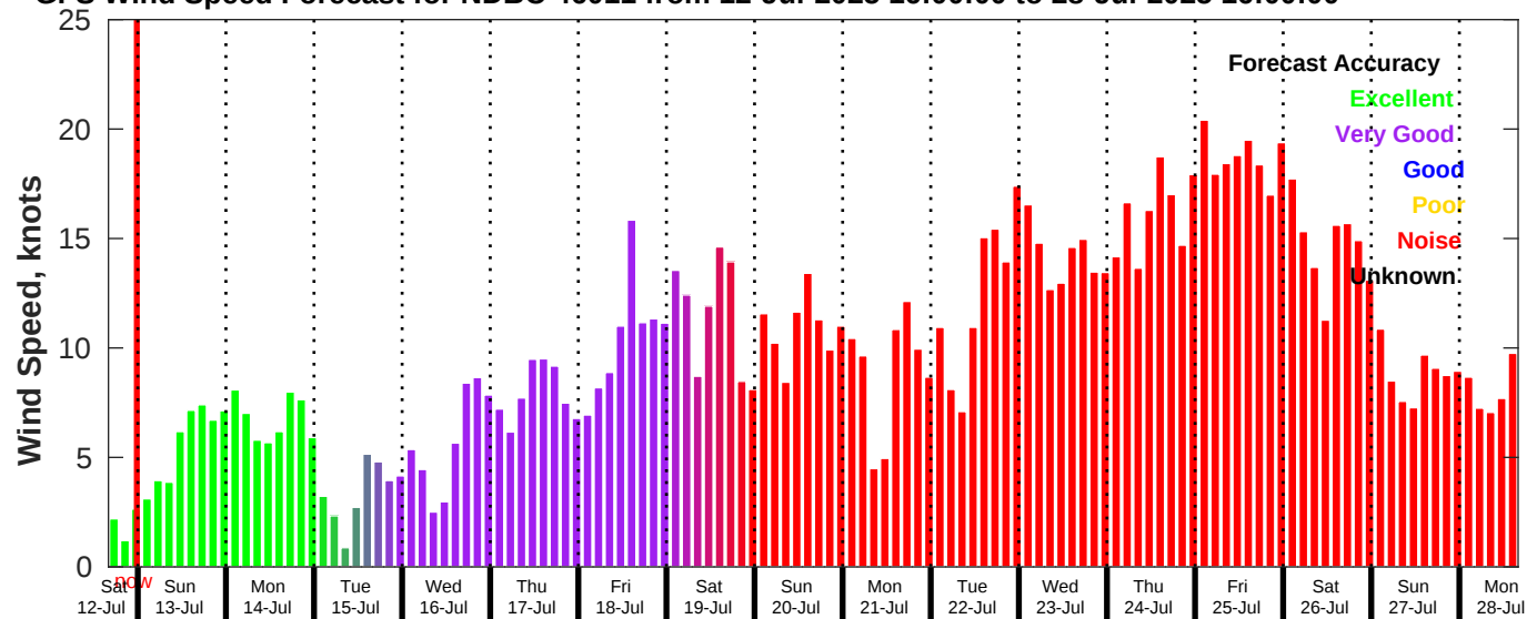
GFS Wind Speed Forecast for NDBC 46011 from 12-Jul-2025 16:00:00 to 28-Jul-2025 16:00:00
